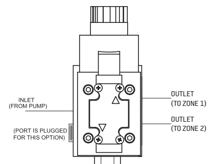
WHEN USED AS A DIVERTER VALVE
